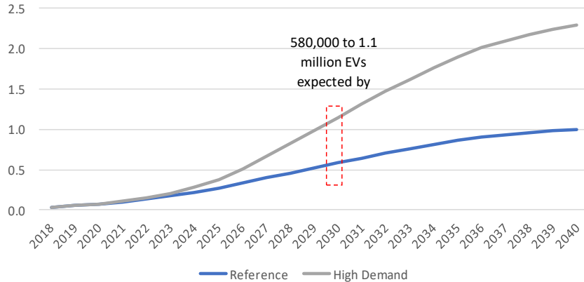
Figure 15: IESO Forecast of Annual EVs in Operation (Million EVs by Year)
