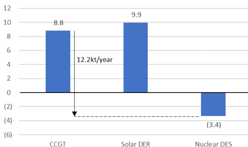
Figure 21: Incremental GHG Emissions Impact of Time Shifting Demand from Mobile Storage (kt/year)
