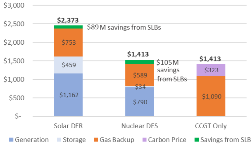
Figure 20: Annual Cost of DER Using Repurposed EV Batteries ($M, 2035)
