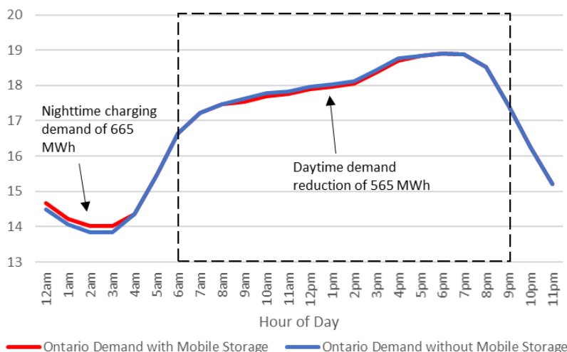
Figure 16: Impact of Mobile Storage on Ontario's Daily Demand Profile (GW by hour; 2035, average summer demand)
